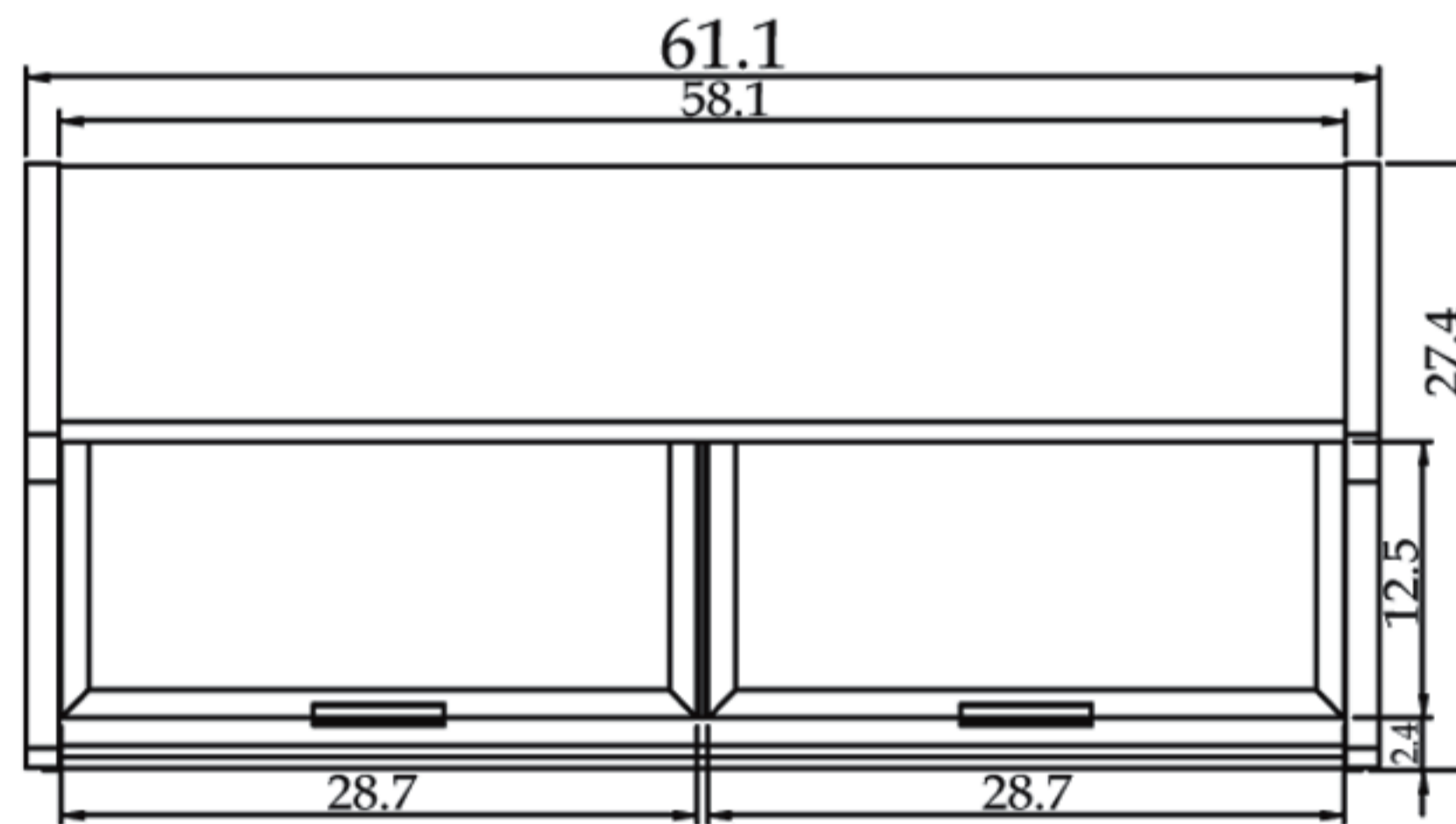
TGF-13F PLAN VIEW
