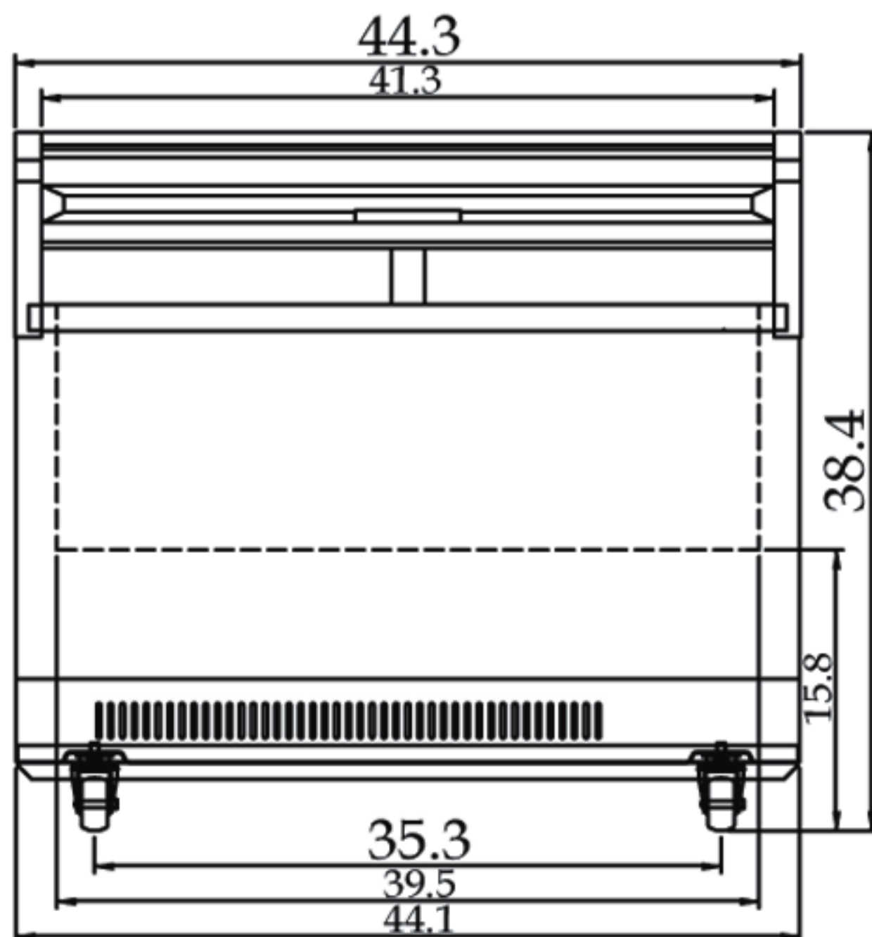
TGF-9F FRONT VIEW
