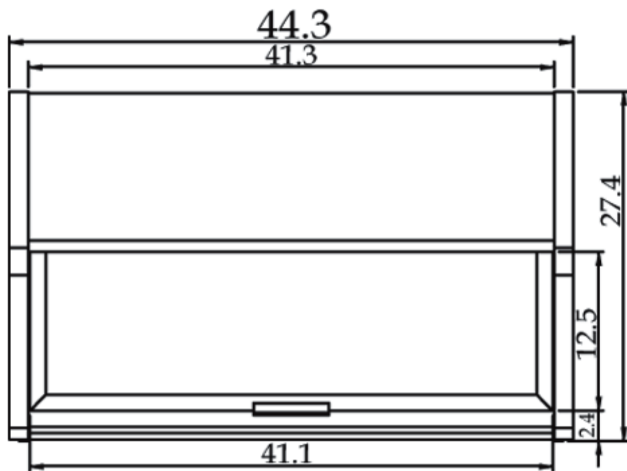
TGF-9F PLAN VIEW
