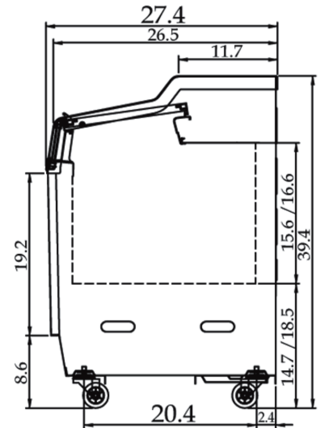
SIDE VIEW
