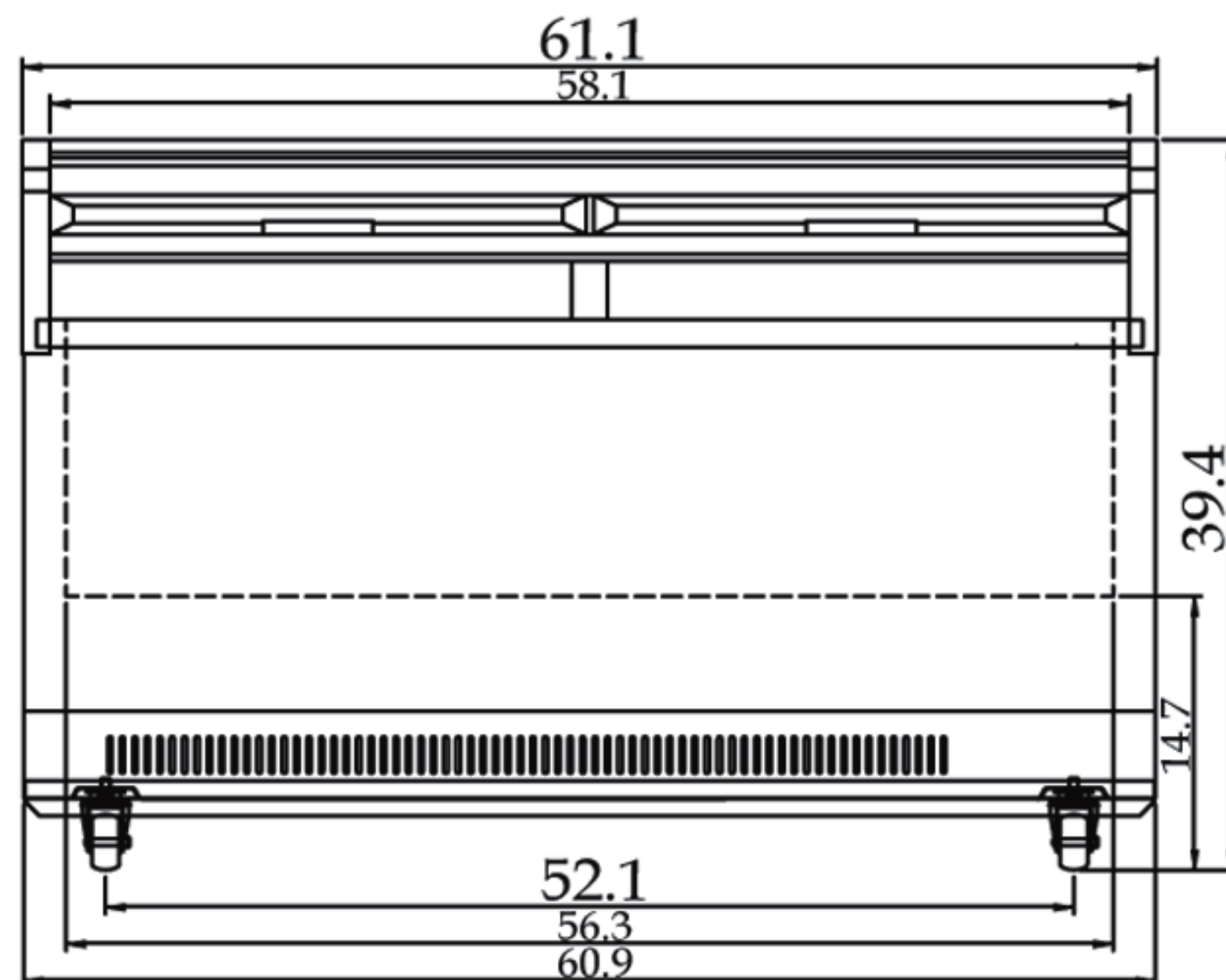
TGF-13F FRONT VIEW
